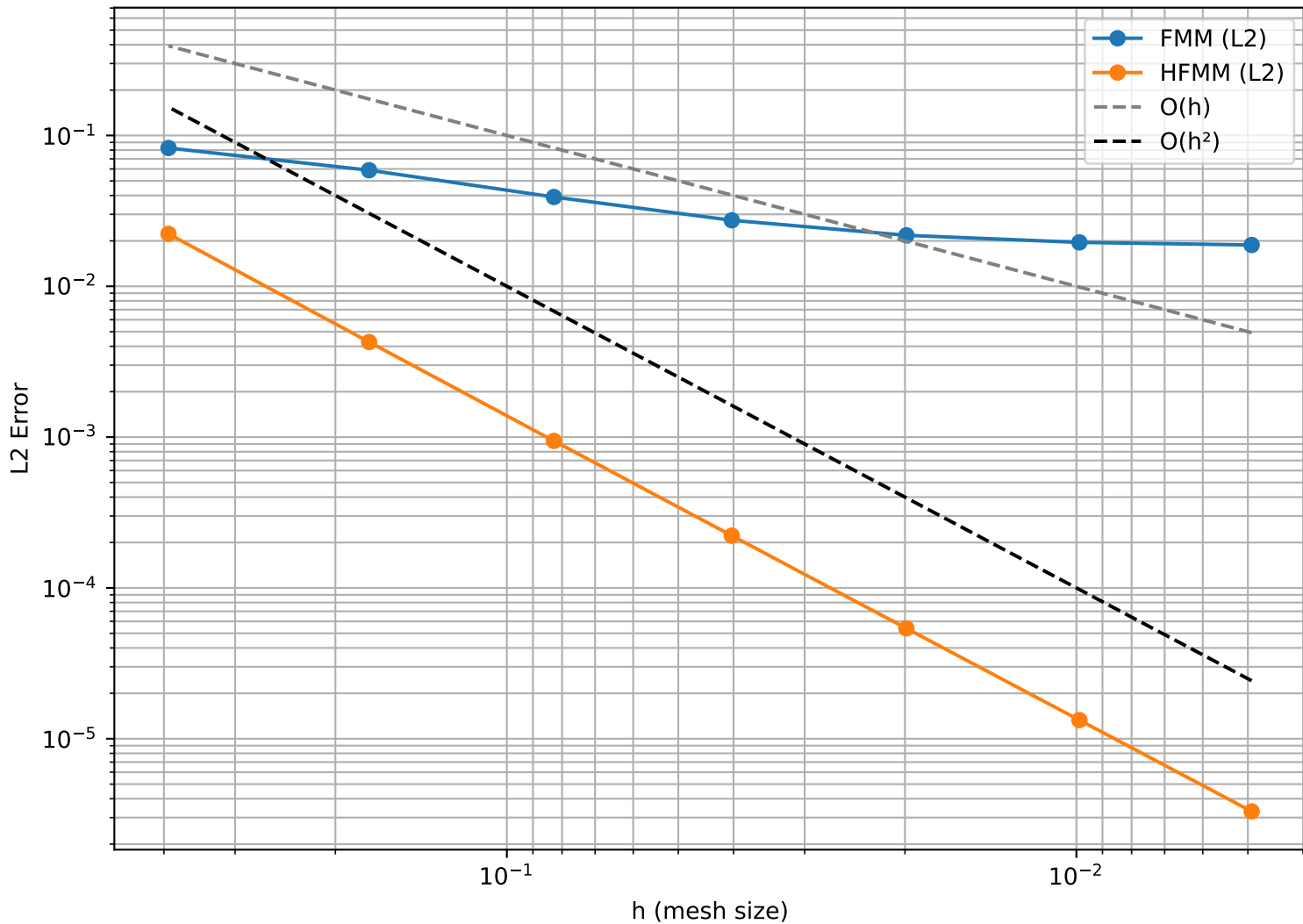
FMM Convergence - Cylinder
